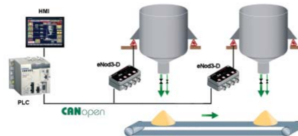
▲ Example of 2 products batching (by unloading)
